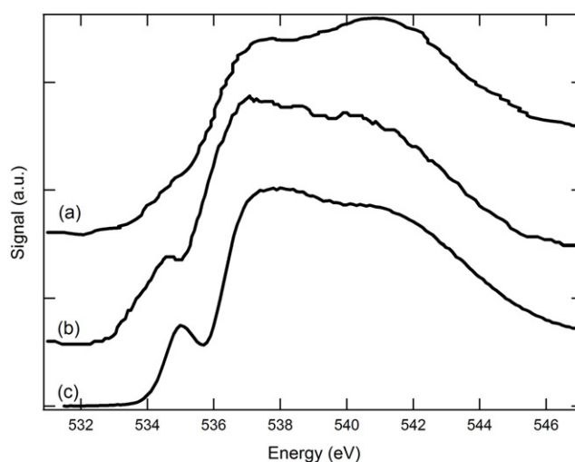
Figure 4. Experimentally observed TEY. (a) The TEY reported in [9] that was obtained around the same time as the ‘old’ TIY. (b) The TEY reported in [1]. (c) A more recent TEY that is known to be correct.
