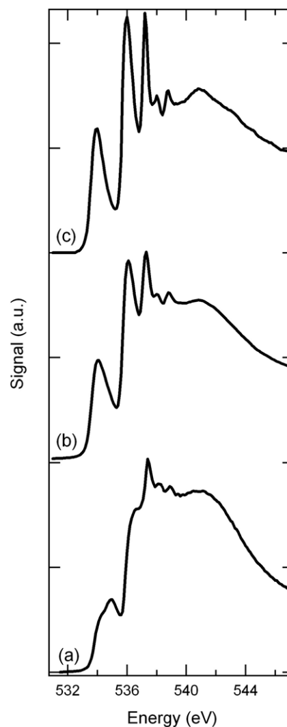
Figure 3. ‘New’ experimental TIY-XA spectra of liquid water for a (a) \sim 20\% vapor contribution, (b) \sim 40\% vapor contribution and (c) \sim 70\% vapor contribution to the observed spectrum.
