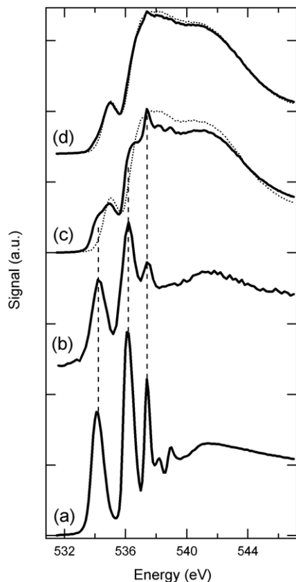
Figure 1. Observed XA spectra of water (solid lines). (a) The TIY spectrum of gas-phase water. (b) The previously observed ‘old’ liquid water TIY spectrum [1, 9]. (c) A more recently obtained ‘new’ liquid water TIY spectrum. (d) The bulk sensitive TEY spectrum of liquid water. The dotted lines show the spectra after vapor subtraction.
